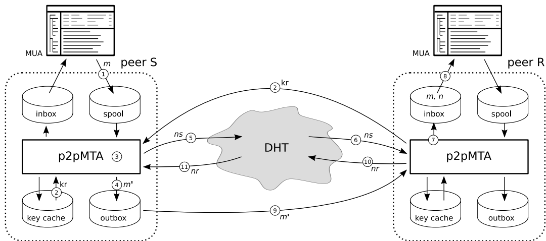
Figure 2: Sending/receiving an e-mail
