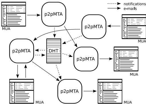
Figure 1: Architecture overview
